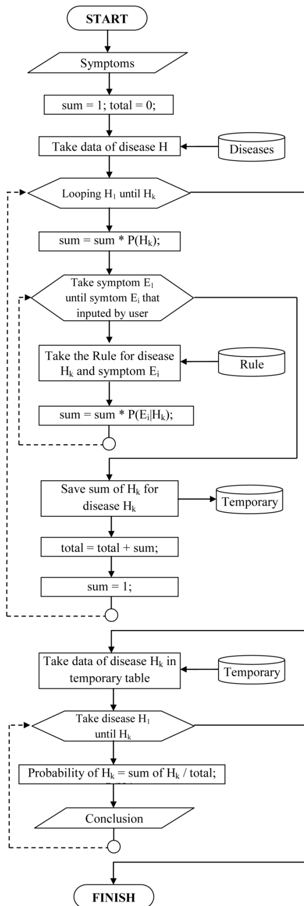
Figure 1. Flowchart Process for Diagnosing Types of Cassava Disease
