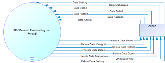
Gambar 1. Context Diagram
