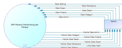
Gambar 1. Context Diagram
